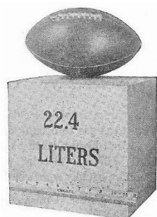
FIG. 19.—The gram-molecular volume (for an ideal gas under standard conditions).
