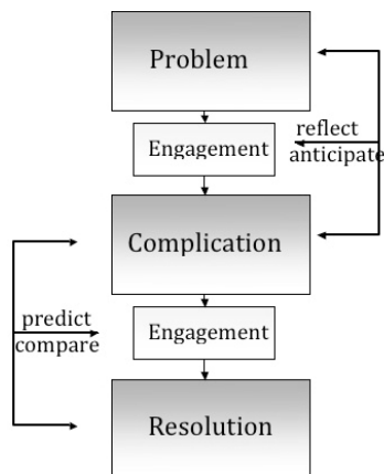
Fig. 1: Story Outline.
